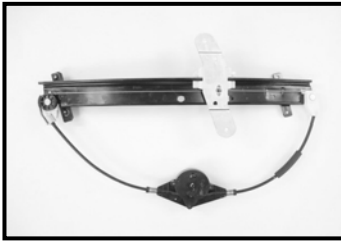
13. ACI Part No 83134 05-92 Ford Crown Victoria, 04-92 Mercury Grand Marquis
