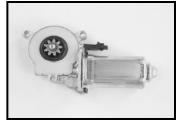
6. ACI Part No 82980 05-84 Cadillac, Chevrolet, GMC, & Oldsmobile
