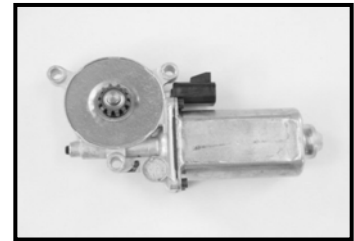
9. ACI Part No 82666 05-96 Chevrolet, 02-96 GMC
