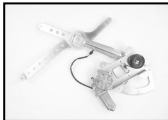
11. ACI Part No 82949 02-88 Chevrolet & GMC
